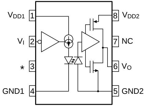
Figure 1. Functional Schematic
